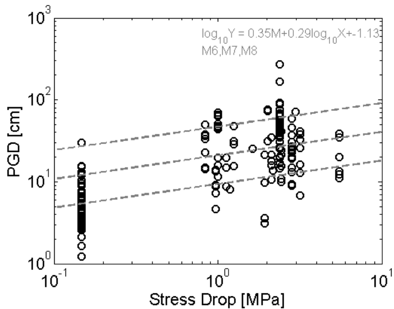
Figure 8.12. Near-source pgd vs stress drop for all records used in this study. The pgd is from high-pass filtered records with a 13 s corner. The three dotted lines represent M 6, 7, and 8 in
