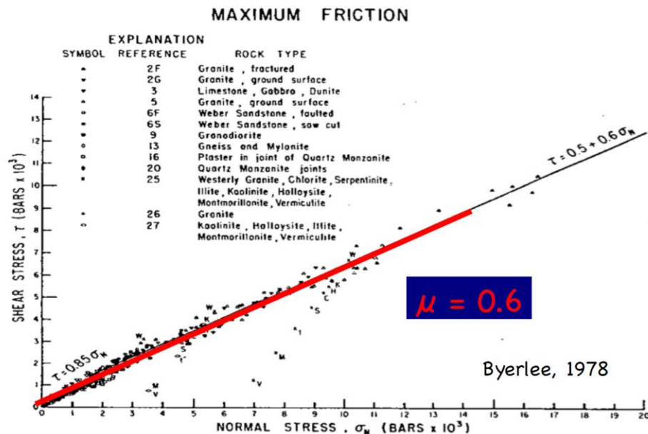
Figure 8.25. Shear stress of frictional yielding of a large range of experiments on different rocks and different normal stresses as reported by Bayerlee. Although there are some notable exceptions (especially clay materials), most rocks have an apparent coefficient of friction of about 0.6. Note that the stress is given in units of kilobars (1kilobar= 100MPa).
