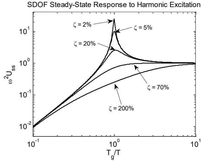
Figure 6.51. Response curves for different damping. There is no resonant peak for damping greater than 71% of critical. Notice that the slope of the log (acceleration response) vs log (period) is approximately linear with increasing driving period. This means that amplitude of the displacement response (i.e., the drift) scales linearly with ground velocity. Also, notice that when the damping is very large, the natural period of the oscillator is not very important. That is, the higher the damping, then the broader the frequency range that response measures velocity.
