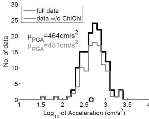
Figure 6.57. This is copied from Yamada, Olsen, and Heaton and it shows the pga for all near-source recordings (JB distance less than 10 km) of earthquakes larger than M 6 for all available data at the time of publication (2004). The grey histogram includes all data prior to the M 7.7 1999 Chi-Chi earthquake, and the black histogram includes the Chi-Chi data. Notice that the addition of Chi-Chi data had a negligible effect on the geometric mean. That is pga saturates at a geometric mean of about \frac{1}{2} g; It seems likely that near-source pga from future earthquakes will also be log-normally distributed about \frac{1}{2} g.
