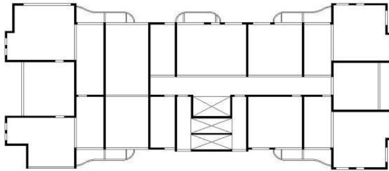
Figure 6.75. Floor plan for a typical Chilean high-rise building. The infilled lines represent reinforced concrete shear wall, whereas the open lines represent non-structural walls. Notice that most architectural walls are also structural shear walls. This is very different from typical US high rises where most architectural walls are not structural walls.
