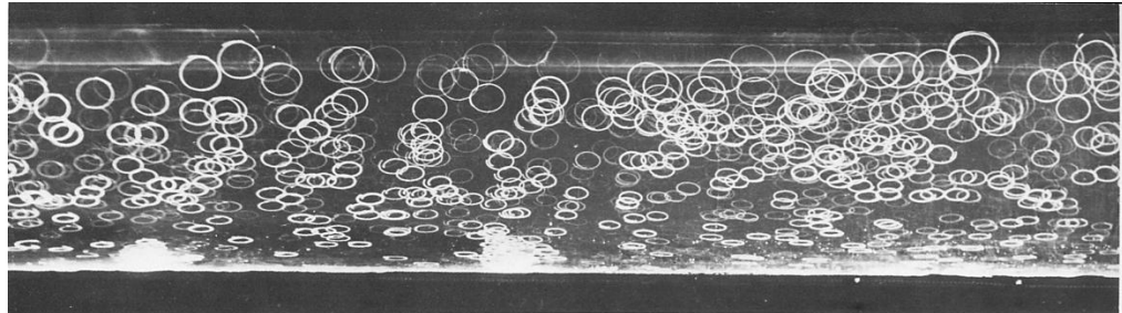
No reflection: pure progressive waves
