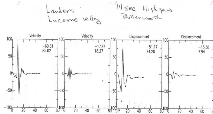
Figure 2.14. Same as 2.13, except that a 14-sec high-pass Butterworth filter has been applied.
