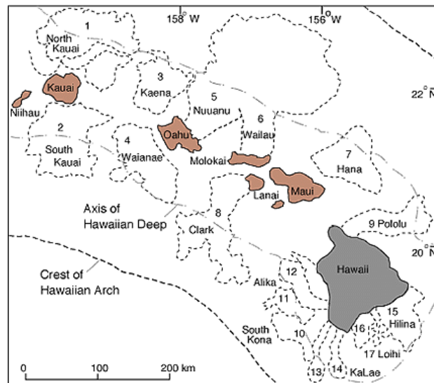
Fig. 8.36. Spatial extent of debris fields created during pre-historic collapse of the flanks of Hawaiian volcanoes. These enormous landslides sometimes ran more than 100 km along the ocean bottom. (Moore and others, 1989)
