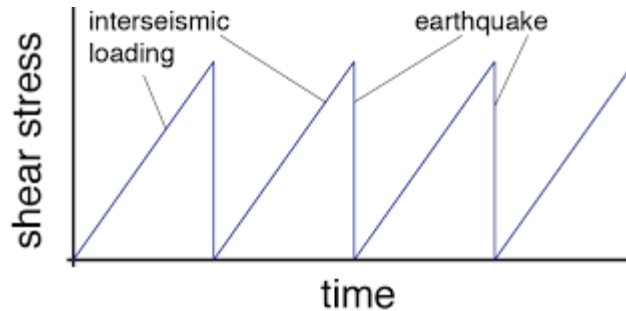
Figure 8.58. Cartoon of the simple Earthquake Cycle
