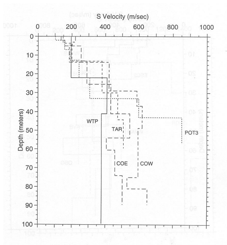
Figure 4.8 Shear-wave velocities for boreholes at stations shown in Figure 4.7
