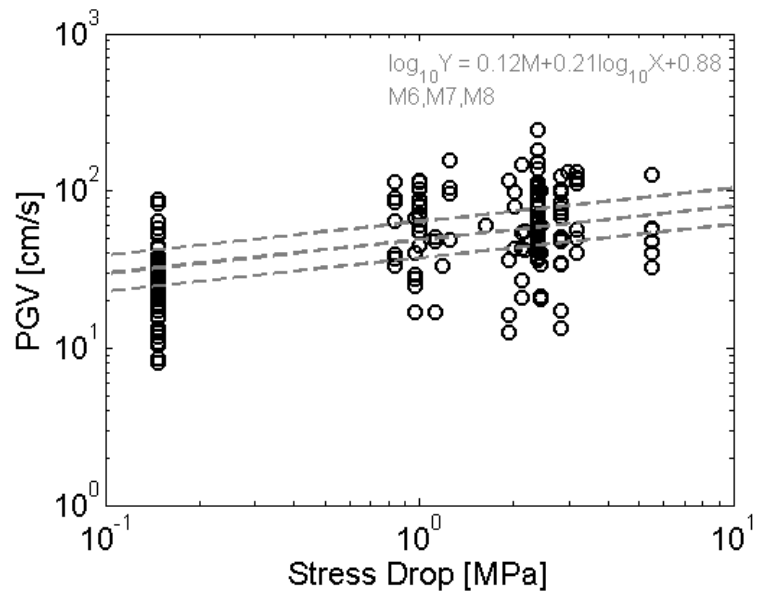
Figure 8.11. Near-source pgv vs stress drop for all records used in this study. The three dotted lines represent M 6, 7, and 8 in the linear least-squares regression
