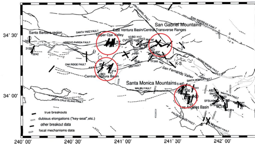
Figure 8-69. Wilde and Stock [1997, J. Geophys. Res. , 102, 4969-4983] plotted inferred maximum horizontal compressive stress, S_H , orientations
