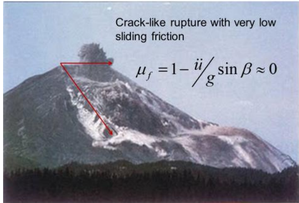
Figure 8.33. Mt. St. Helens during the massive landslide that depressurized the magma chamber.
